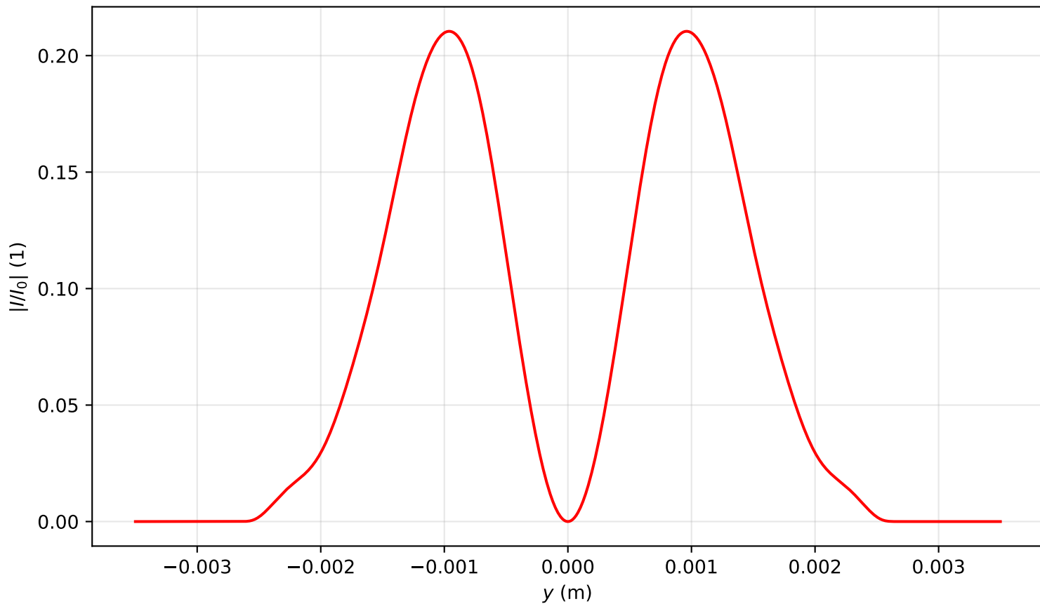
Intensity profile I(x=0, y, z=3.423)/I_0 , P_{in}=0.5P_{cr} , artificial time
